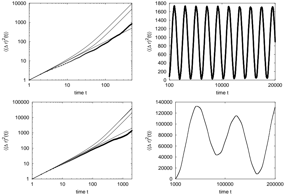
Fig. 4. Mean square displacement for quantum multi-baker with phases \varphi_q = \varphi_p = 1/2 for N = 50 (top row) and N = 200 (bottom row). The left plots show the short time behavior on the log-log scale. We see the same diffusive behavior as in the generic case. The right plots are normal scale and show the oscillations encountered on the long scale. All the plots are numerical evaluations of the exact formula (26).
